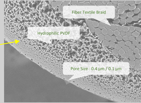
Membrane Cross Section Expansion
