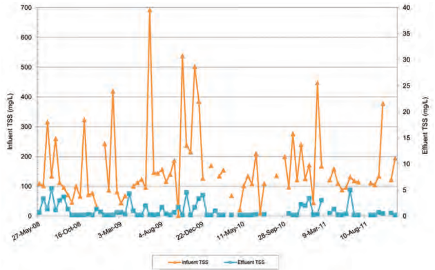
Figure 4: Influent and Effluent TSS (note: all non-detect permeate samples were assumed to be 0.2 mg/L)
